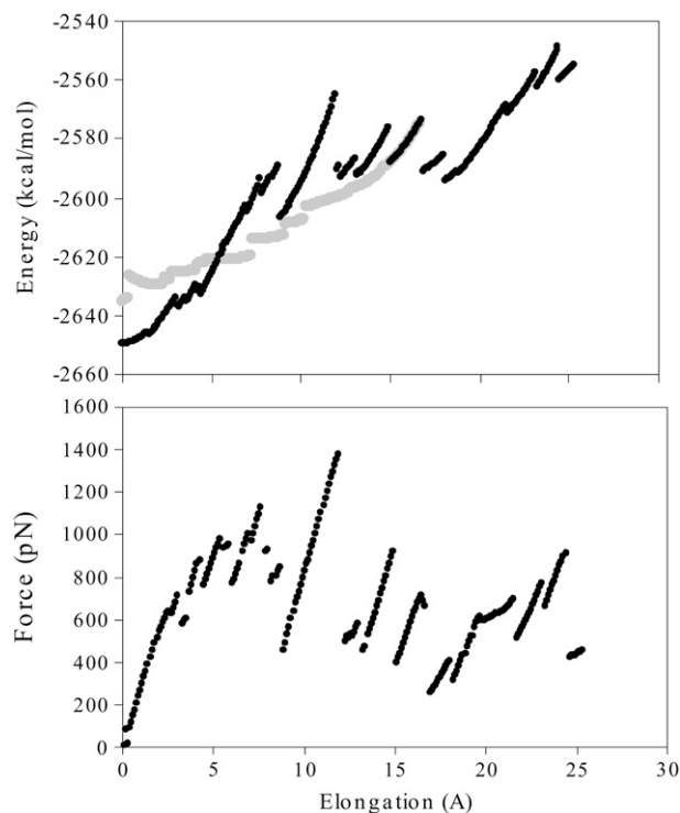
FIGURE 2 Properties of energy minima of Ig27 during stretching. (a) Energy. Note that gray lines are results as stretching is reversed. (b) Force.
